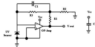
Fig. 7 Application circuit
