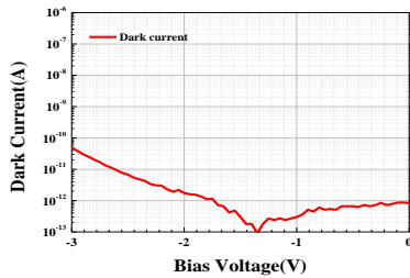
Fig. 4 Dark current of UVB sensor (Log scale)
