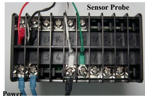
Fig.1.2 Wiring digram of MG-02 (I-out)
