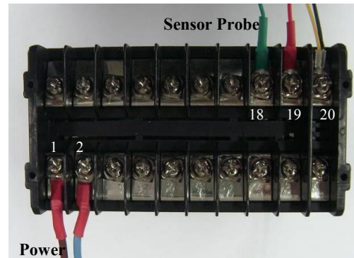
Fig2. Wiring digram of MG-05 (Vout)
