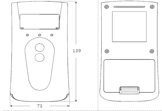
Fig2. Size of Radiometer 7.1 (Unit : mm)
