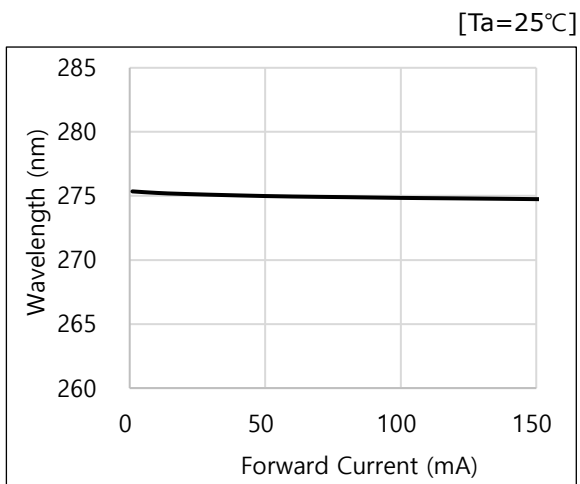
3) Peak Wavelength vs. Forward Current
